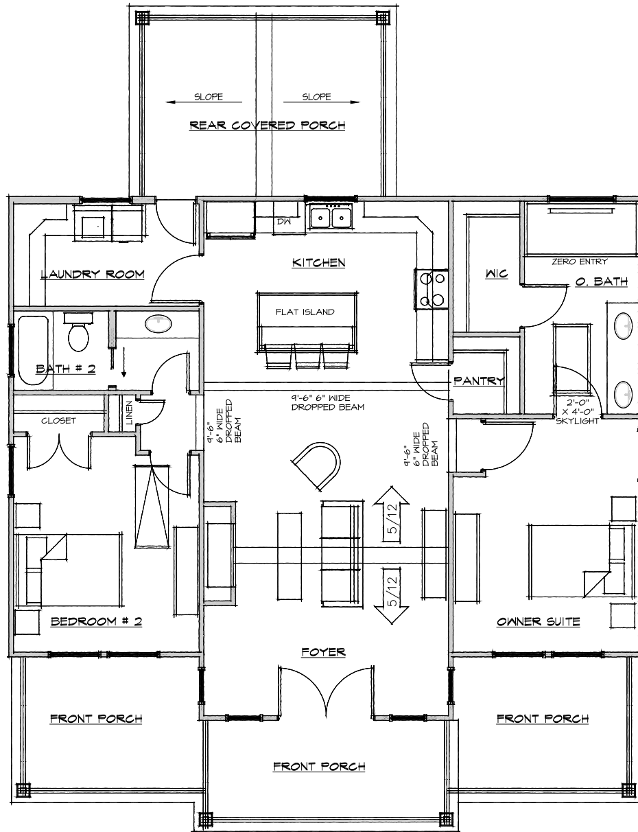
First Floor Plan W/ Extended Front Porch
